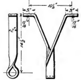
Figs. 253-254. Throttle Stem Bracket.
